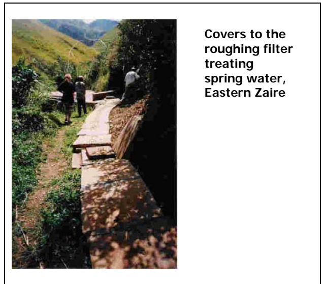
Spring box with roughing filter on the outlet (to the right) prior to the water entering the pipeline
